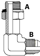
BSPTM x JICM Elbow 90° EXT
