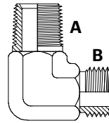
NPTM x ORFSM 90° Elbow
