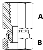
BSPTF x BSPPFS Adaptor
