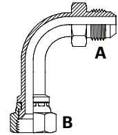
JICM x JICFS 90° Long Bend
