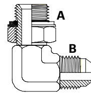
BSPPM x JICM 90° Elbow
