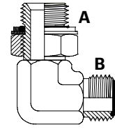
BSPPM x ORFSM 90° Elbow
