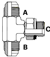
JICM x JICM x BSPPM Tee
