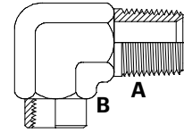
BSPTM x BSPTF 90° Elbow
