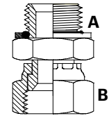
BSPPM x JICFS Adaptor
