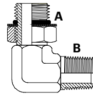
UNOM x BSPTM 90° Elbow
