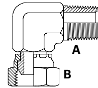
BSPTM x BSPPFS 90° Elbow
