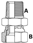
BSPTM x JICFS Adaptor
