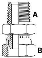
BSPTM x BSPPFS Adaptor
