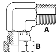
NPTM x NPTFS 90° Elbow
