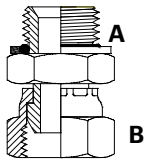
BSPPM x BSPPFS Nipple
