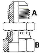
J1CM x J1CFS Adaptor
