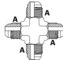
JICM Cross
