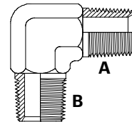
NPTM x NPTM 90° Elbow
