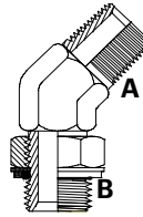
BSPTM x BSPPM 45° Elbow
