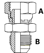
BSPPFs x JICM Adaptor
