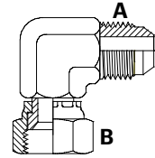
J1CM x J1CFS 90° Elbow
