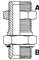
BSPPMBH x BSPPM
