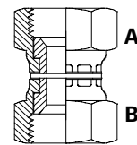
J1CFS x J1CFS Adaptor
