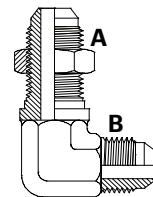
JICMBH x JICM 90° Elbow
