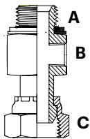
BSPPM x BSPTF x BSPPFS Test Point Adaptor
