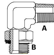
BSPTM x BSPPM 90° Elbow
