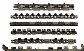
ADAPTED TRANSMISSION CHAINS
